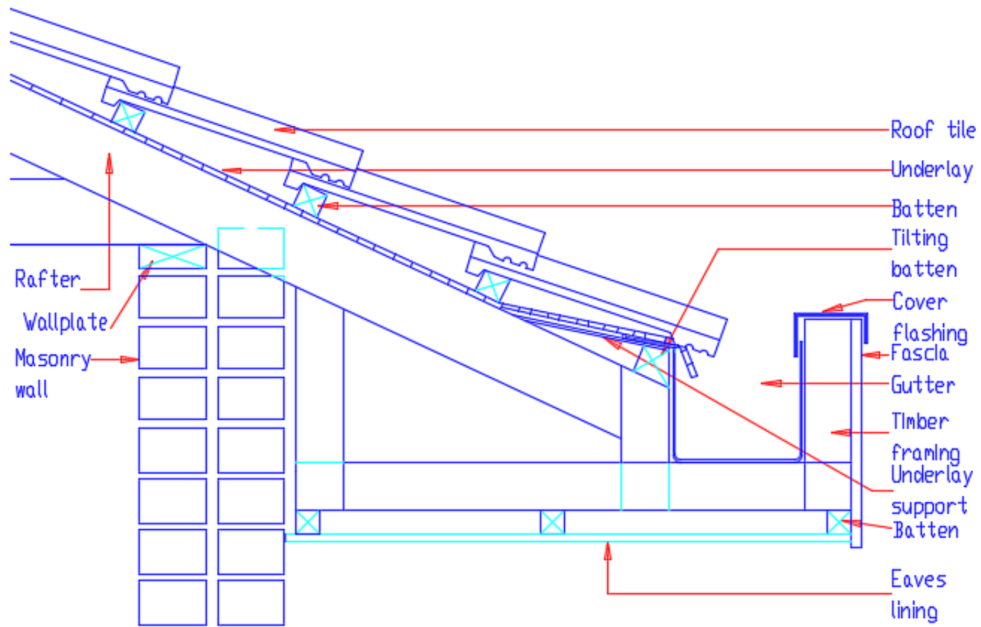
EAVES WITH CONCEALED GUTTER
